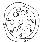
VIEW A SCALE 2.5
