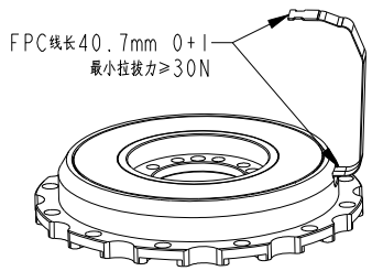
DRAWING IN THIRD ANGLE PROJECTION
